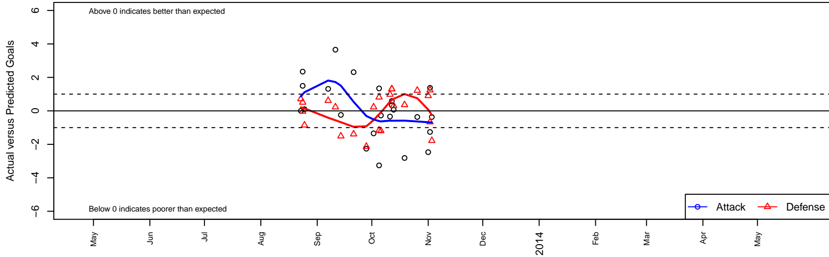
FC Nova Grey G00 Dots are actual minus expected GF (blue circles) and GA (red triangles). Blue line is smoothed change in attack strength. Red is smoothed change in defense strength.
